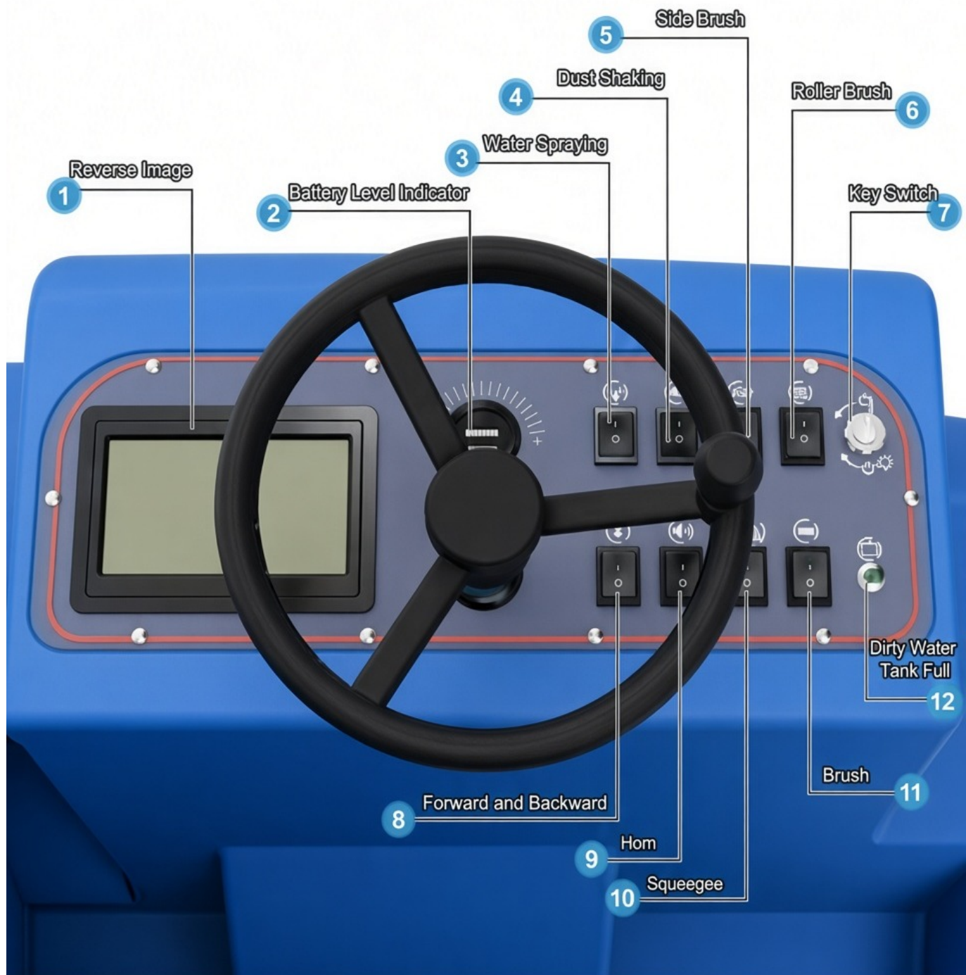
A90RC multi-function control panel.
